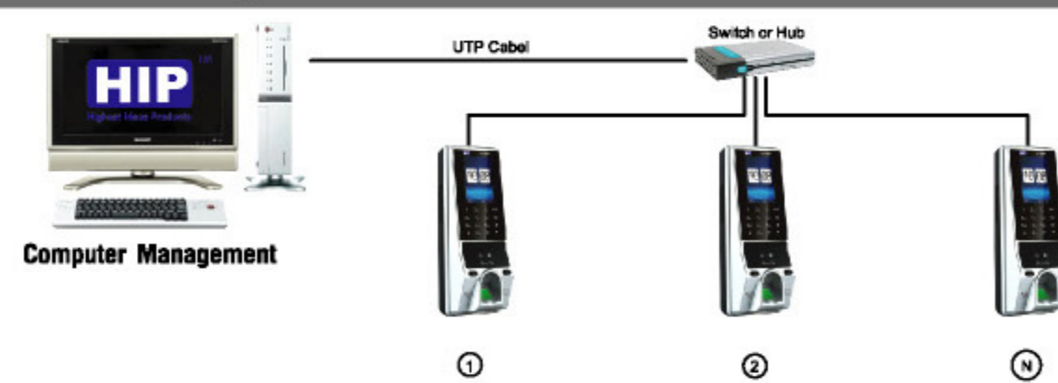
Computer Management
